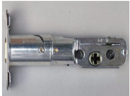
2-3/4" (70mm)
